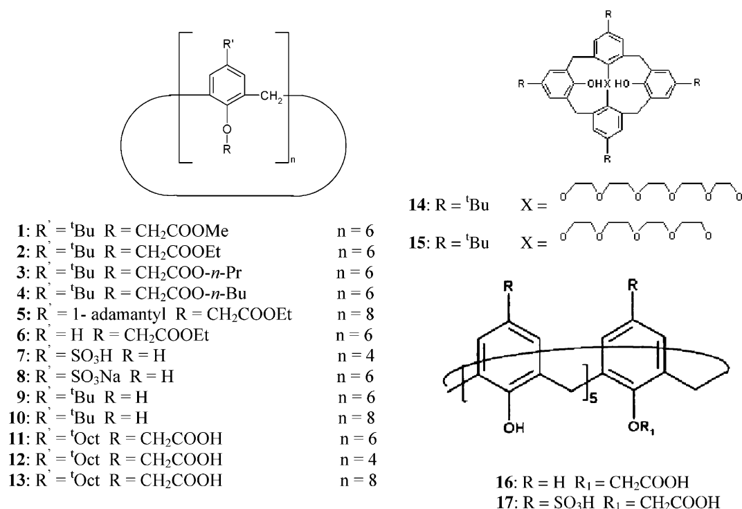
Chart 1. The structure of calix [n]arenes involve in experiments.
